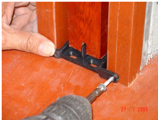
12. Fix plastic floor guide to side door jamb
